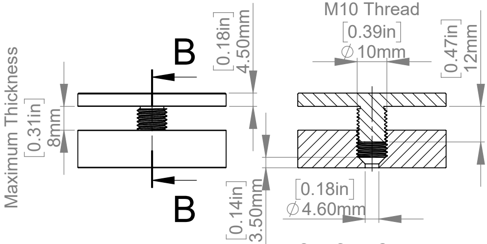
SECTION B-B SCALE 1 : 1.25
