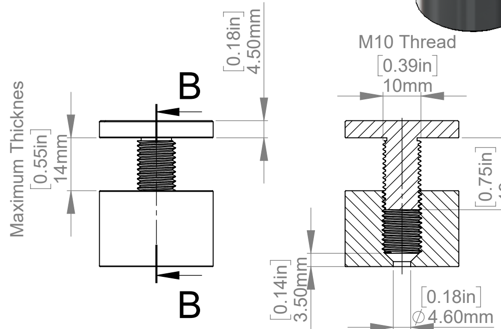
SECTION B-B
