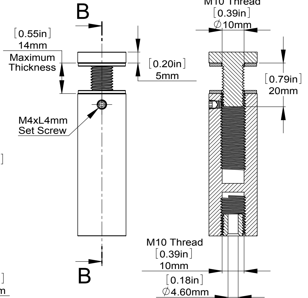
SECTION B-B
