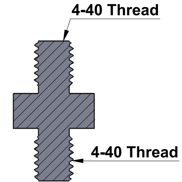
SECTION S-S
