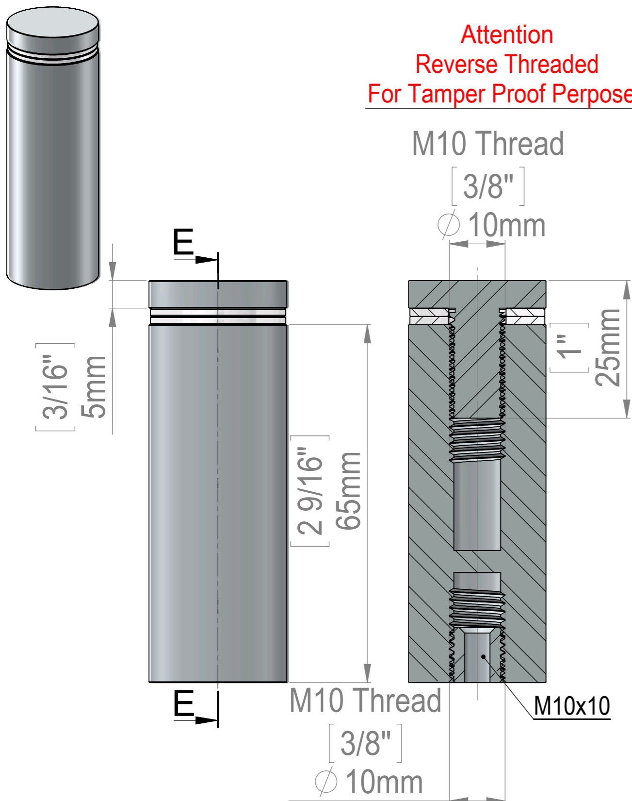
SECTION E-E SCALE 1.5 : 1
