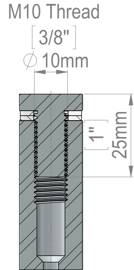
SECTION E-E SCALE 1.5 : 1
