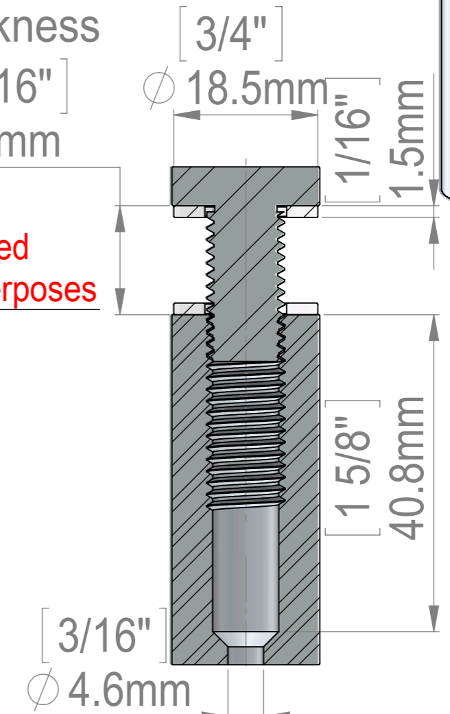
SECTION F-F SCALE 1.5 : 1
