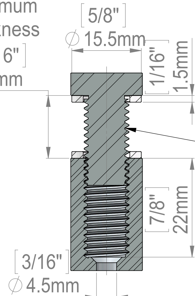
SECTION E-E SCALE 2 : 1 M10 Thread
