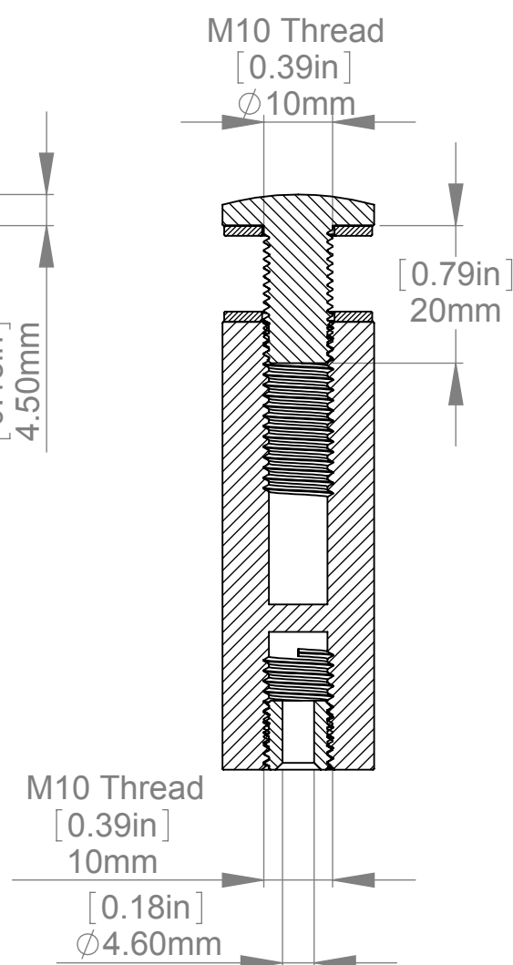
SECTION B-B
